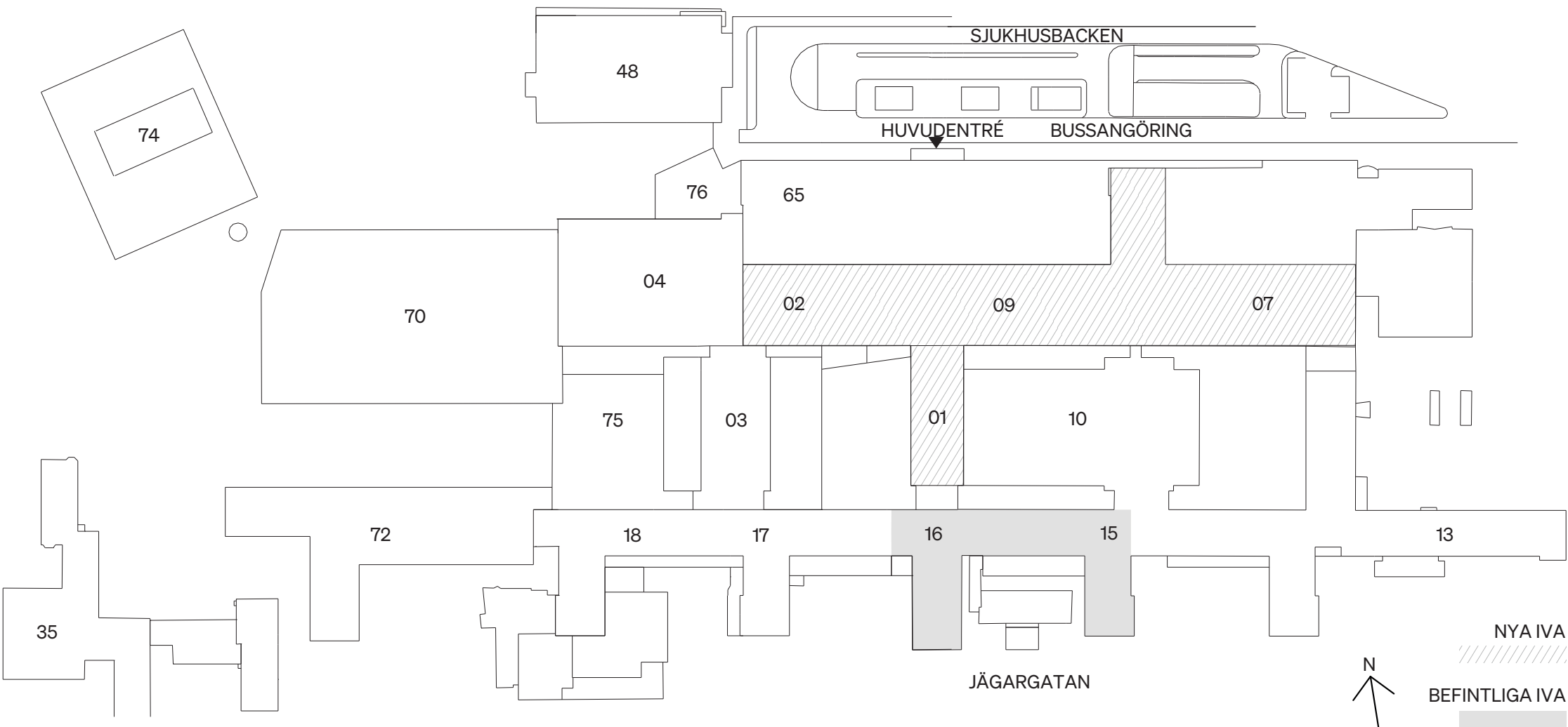
Situationsplan - Sös
